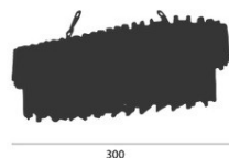
Chandelier P161 Brand : Lamp & Light Designed lamp for your decoration Dimension : W300 x H450 (Suspension length 1200mm) Lamp Type : E14 x 9 PCS (Please Use Super bright bulb E27) Material : K9 Crystal, Steel Color : Gold/Chrome, Clear Crystal Weight : 20 KG
