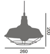
Q166 Dimension: 260x260x200mm Material: Steel Color: Black
